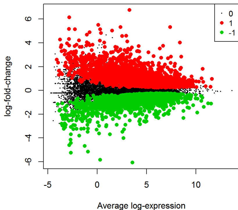
M-A plot (Minus, Add)
